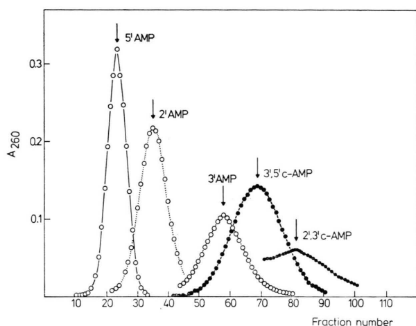
Fig. 3. Separation of the different mononucleotides by ion-exchange chromatography with a Dowex 1 \times 2 (200–400 mesh, Cl - form) column with 2.5 mM HCl as eluting fluid.
